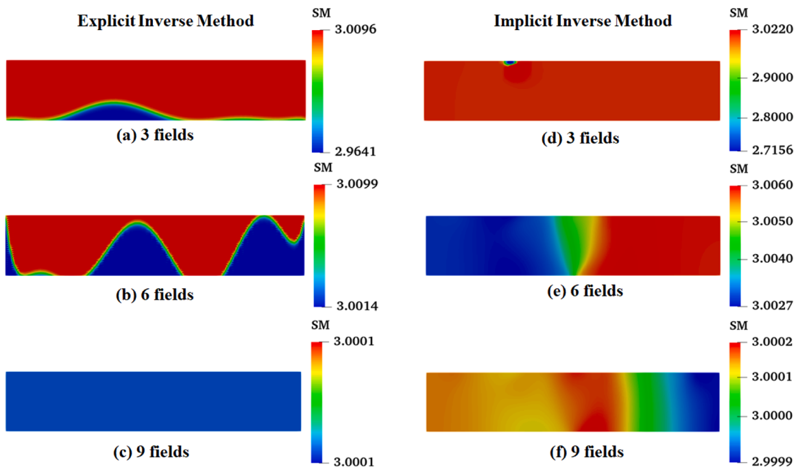
Fig. 14. The reconstructed results with varying 3,6 and 9 surface displacement datasets corresponding to Sample 1 (5 % noise is introduced into the measured data, Unit: MPa).
