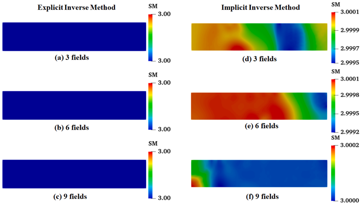
Fig. 8. The reconstructed results with varying 3,6 and 9 surface displacement datasets corresponding to Sample 1 (Without noise, Unit: MPa).
