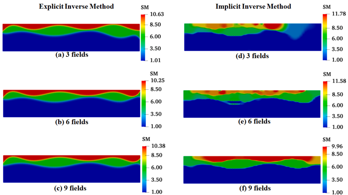
Fig. 13. The reconstructed results with varying 3,6 and 9 surface displacement datasets corresponding to Sample 3 (1 % noise is introduced into the measured data, Unit: MPa).
