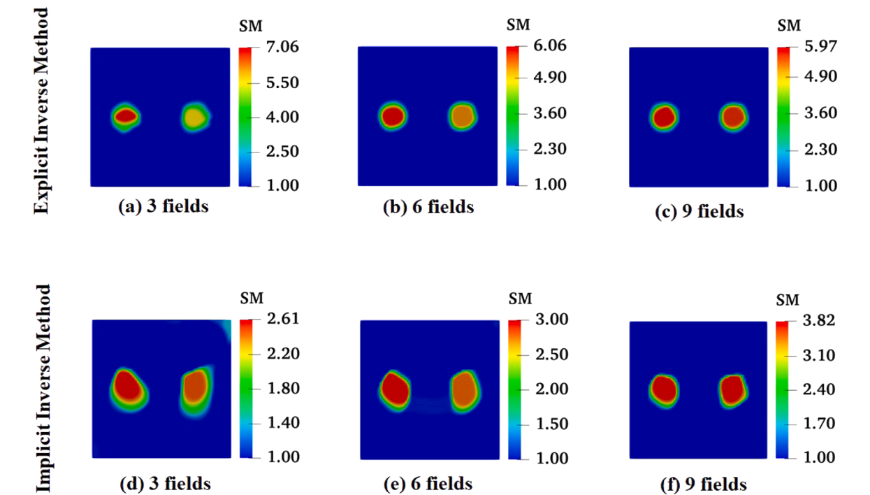
Fig. 26. The reconstructed results with varying 3,6 and 9 surface displacement datasets corresponding to Sample 2 (Without noise, Unit: MPa).
