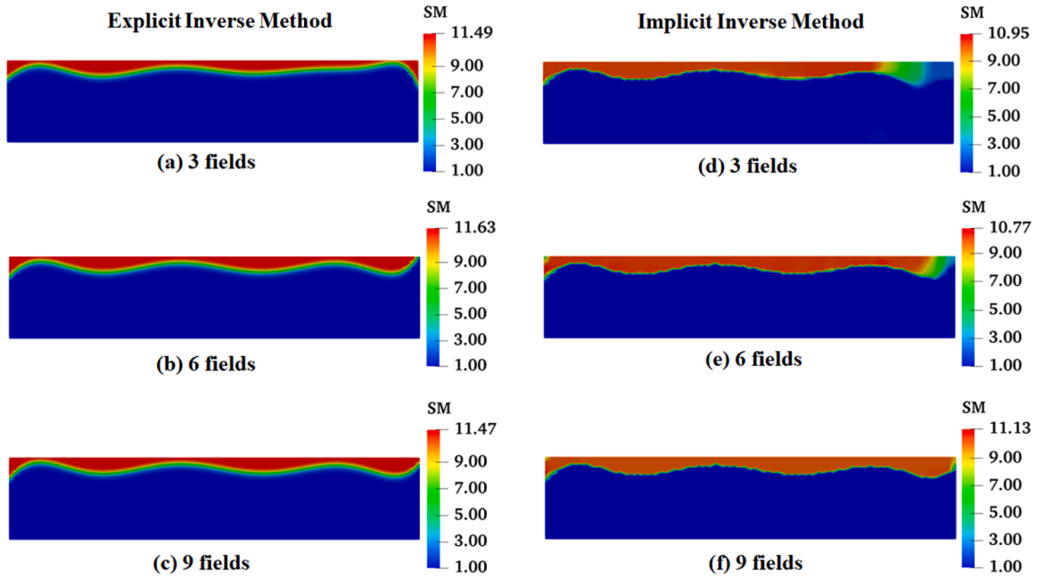
Fig. 9. The reconstructed results with varying 3,6 and 9 surface displacement datasets corresponding to Sample 2 (Without noise, Unit: MPa).
