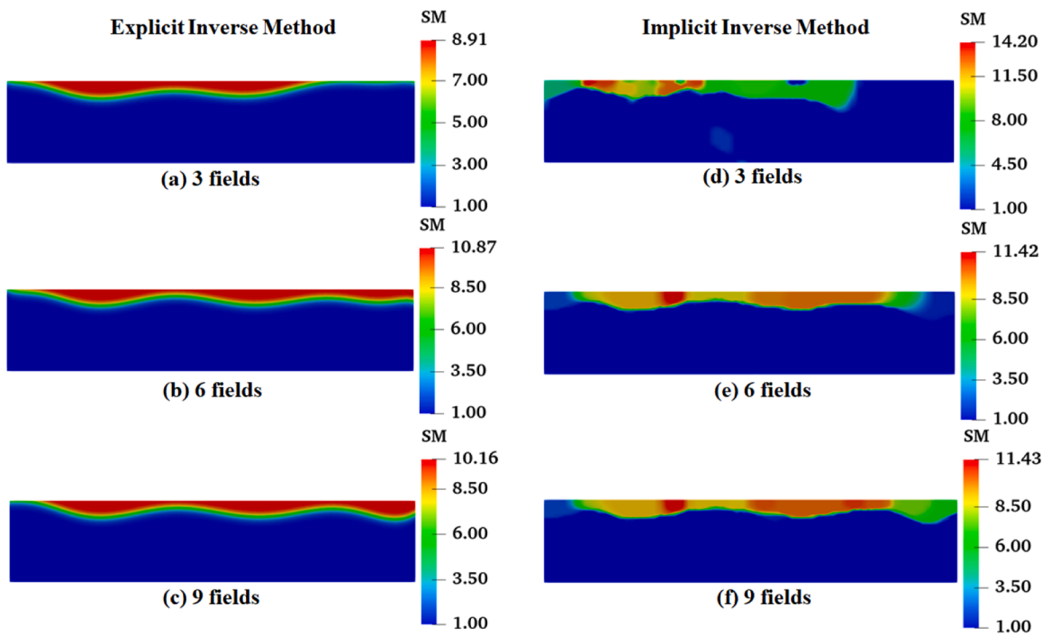
Fig. 15. The reconstructed results with varying 3,6 and 9 surface displacement datasets corresponding to Sample 2 (5 % noise is introduced into the measured data, Unit: MPa).
