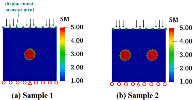
Fig. 21. Target shear modulus distribution of composite with inclusions embedded (Unit: MPa).
