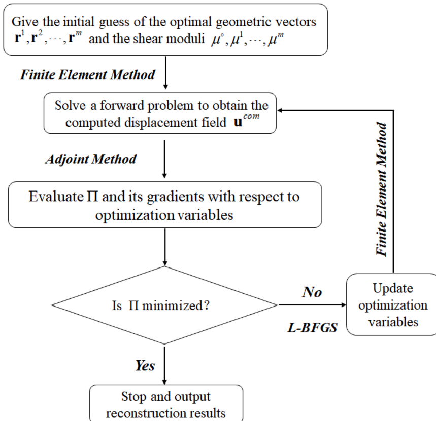
Fig. 5. The flow chart of the proposed explicit inverse method.
