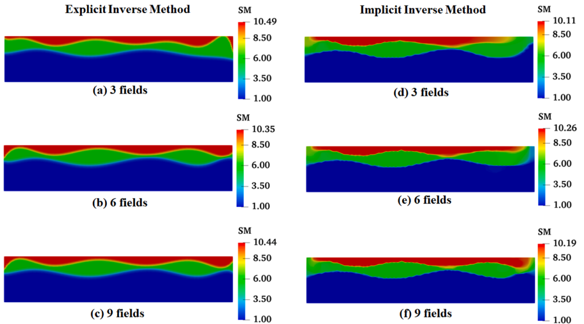
Fig. 10. The reconstructed results with 3,6 and 9 surface displacement datasets corresponding to Sample 3 (Without noise, Unit: MPa).
