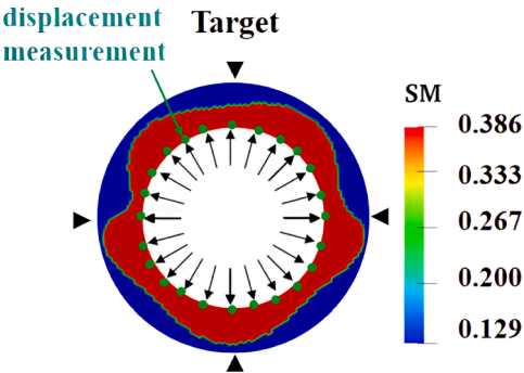
Fig. 17. Target shear modulus distribution of a bilayer ring structure (Unit: MPa).
