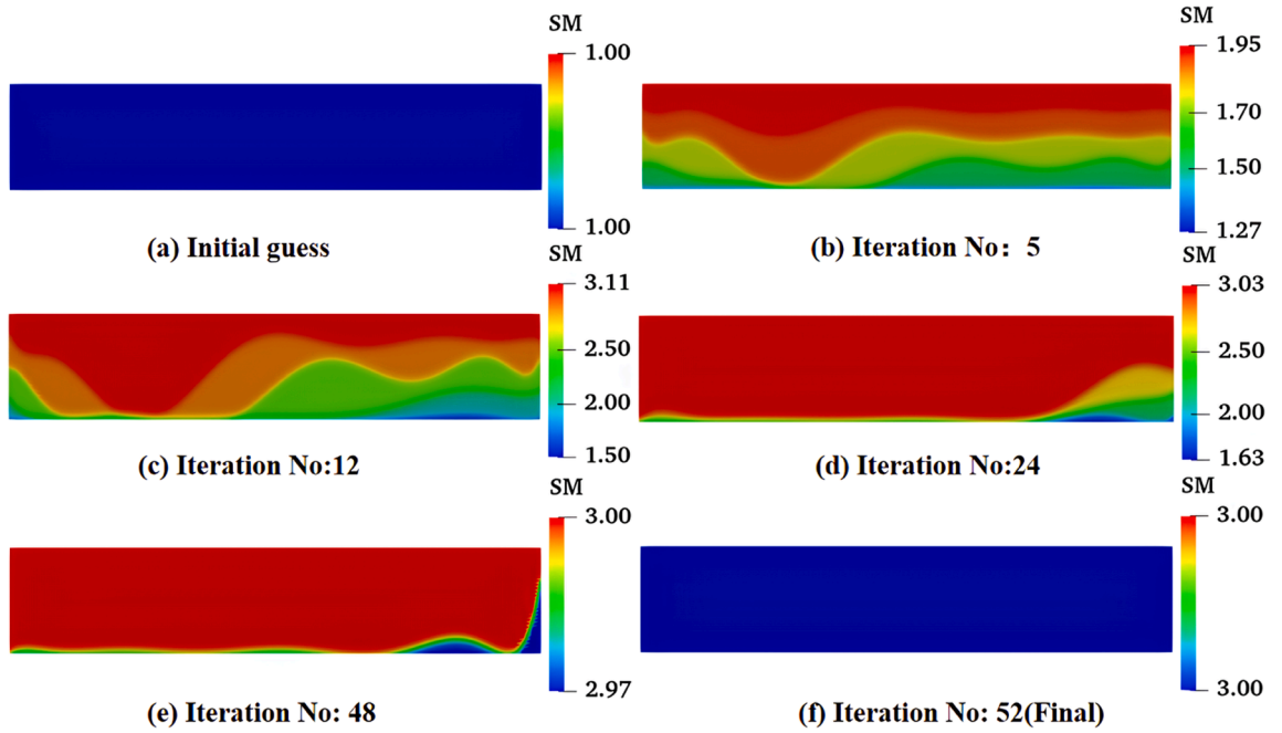
Fig. 7. The optimization process with six layers initially utilizing the explicit inverse scheme for Sample 1 (Without noise, Unit: MPa).
