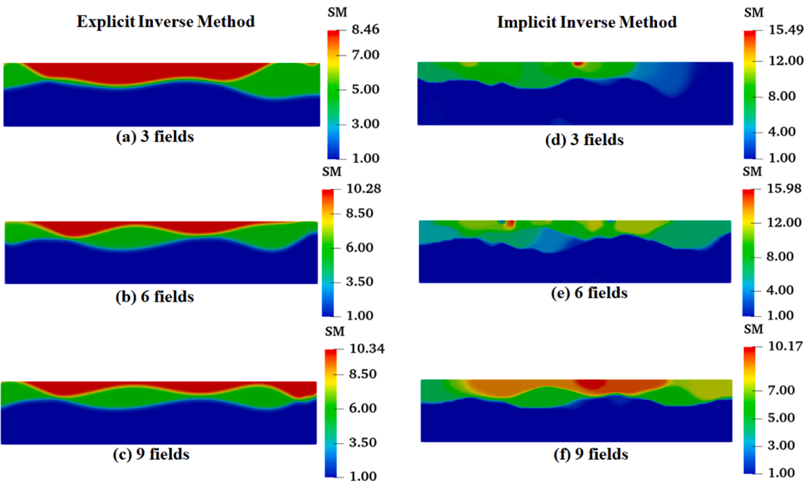
Fig. 16. The reconstructed results with varying 3,6 and 9 surface displacement datasets corresponding to Sample 3 (5 % noise is introduced into the measured data, Unit: MPa).
