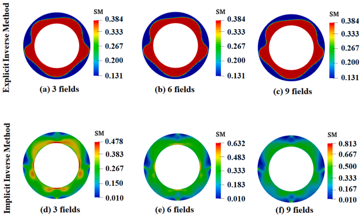
Fig. 19. The reconstructed results with varying 3, 6 and 9 surface displacement datasets (Without noise, Unit: MPa).
