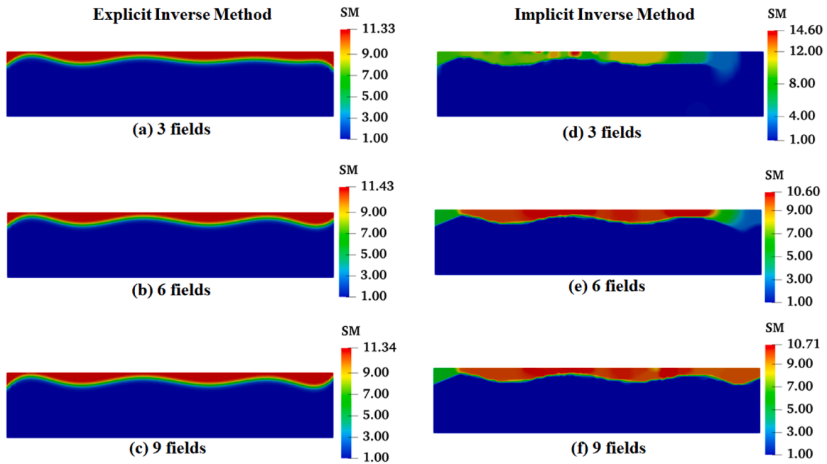
Fig. 12. The reconstructed results with varying 3,6 and 9 surface displacement datasets corresponding to Sample 2 (1 % noise is introduced into the measured data, Unit: MPa).
