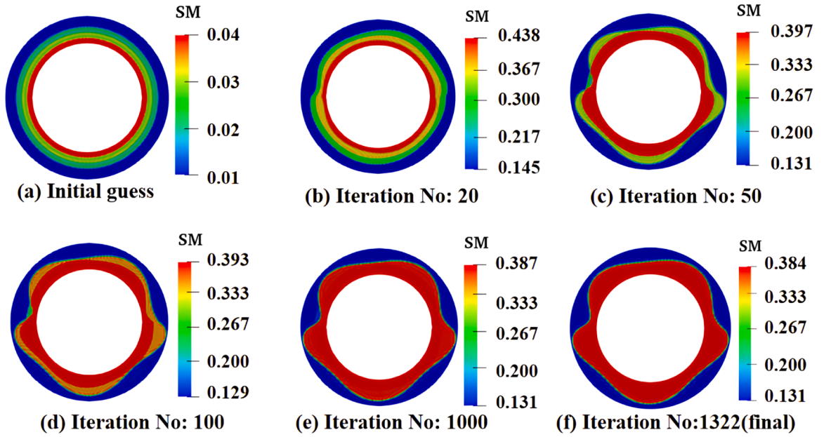
Fig. 18. The optimization process with four layers initially utilizing the explicit inverse scheme with 3 surface datasets (Without noise, Unit: MPa).
