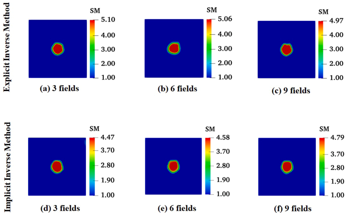
Fig. 23. The reconstructed results with varying 3,6 and 9 surface displacement datasets corresponding to Sample 1(Without noise, Unit: MPa).
