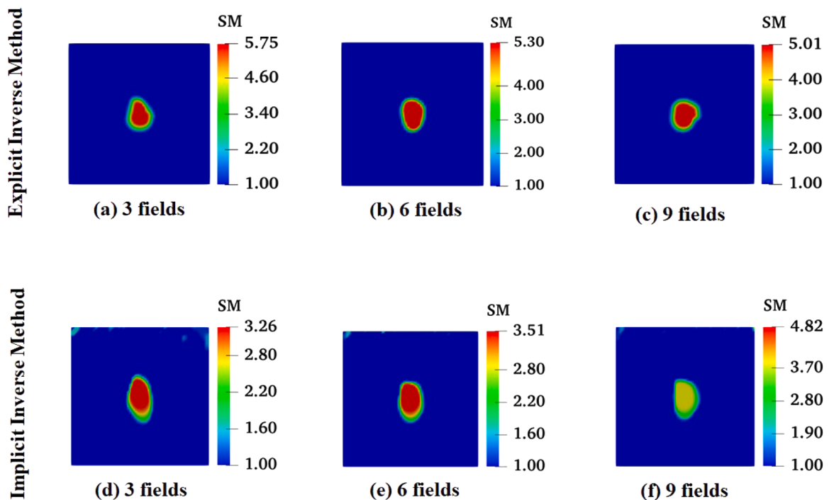
Fig. 24. The reconstructed results with varying 3, 6 and 9 surface displacement datasets corresponding to Sample 1 (1 % noise is introduced into the measured data, Unit: MPa).
