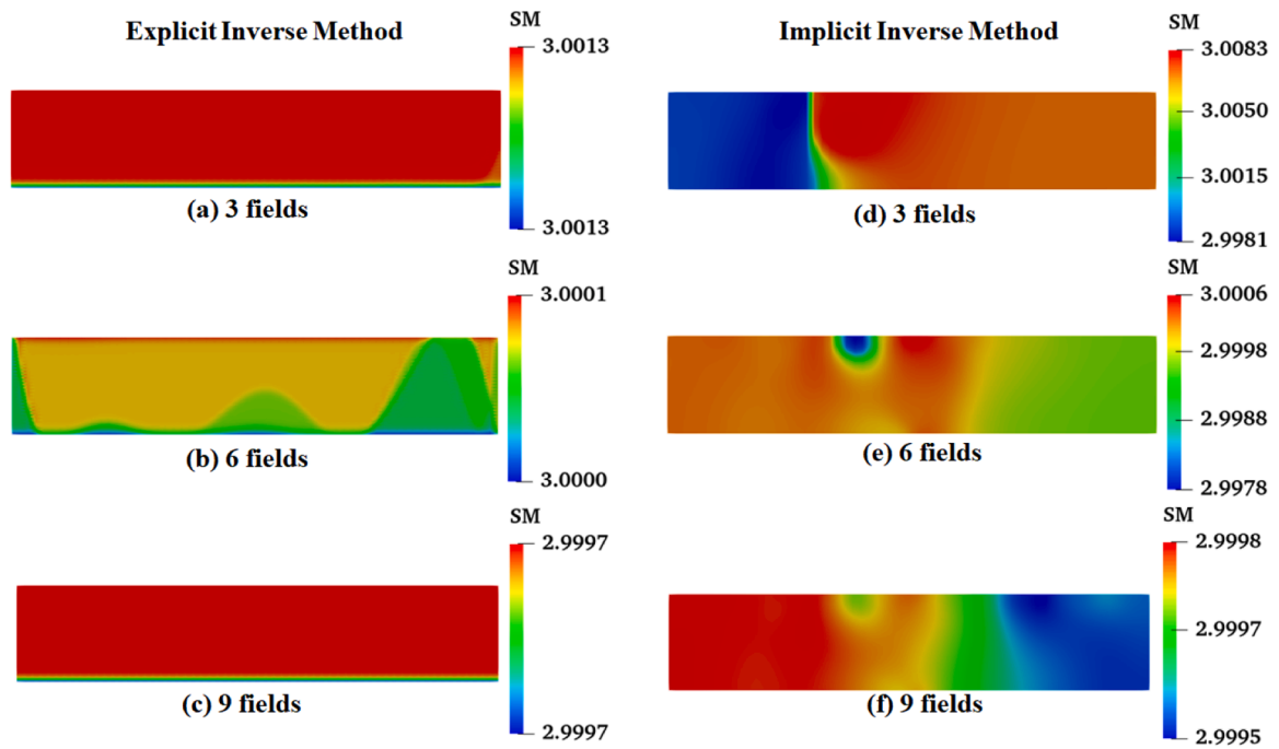
Fig. 11. The reconstructed results with varying 3, 6 and 9 surface displacement datasets corresponding to Sample 1 (1 % noise is introduced into the measured data, Unit: MPa).
