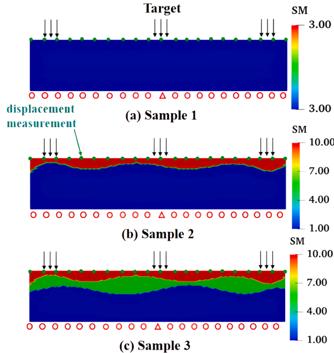
Fig. 6. The target shear modulus distribution of three samples with different number of layers (Unit: MPa). SM stands for shear modulus.
