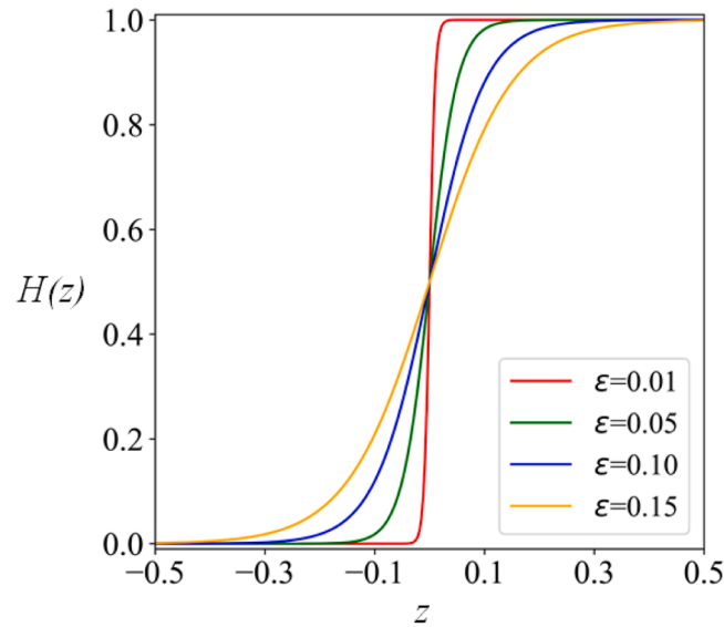
Fig. 4. An approximation of Heaviside function.
