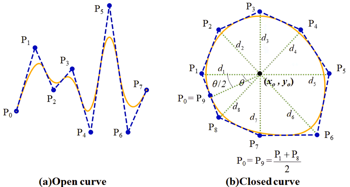
Fig. 1. Two examples of the curve expressed by B-spline functions.
