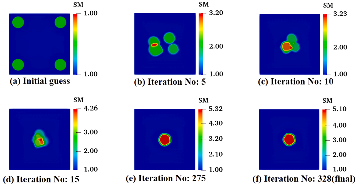
Fig. 22. The optimization process with four inclusions initially utilizing the explicit inverse scheme for a solid with inclusion embedded when 3 surface displacement datasets are utilized (Without noise, Unit: MPa).
