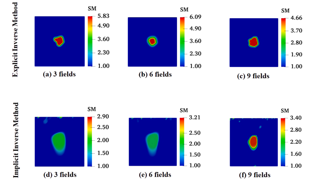
Fig. 25. The reconstructed results with varying 3,6 and 9 surface displacement datasets corresponding to Sample 1 (5 % noise is introduced into the measured data, Unit: MPa).
