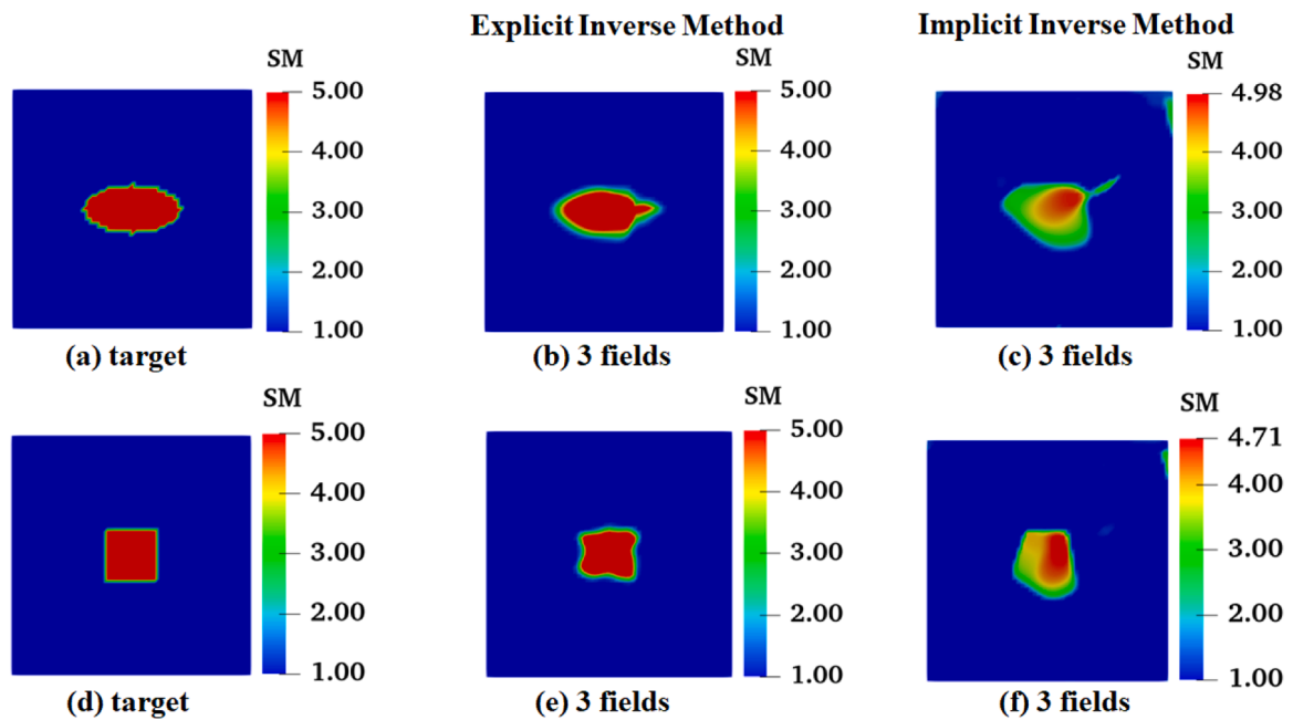
Fig. 27. The target and reconstructed results for varying shapes of inclusion with 3 displacement datasets corresponding to Sample 1 (Without noise, Unit: MPa).
