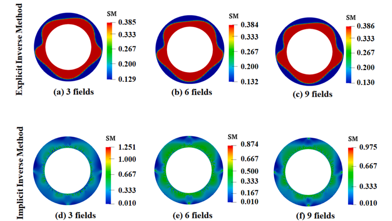
Fig. 20. The reconstructed results with varying 3,6 and 9 surface displacement datasets (1 % noise is introduced, Unit: MPa).
