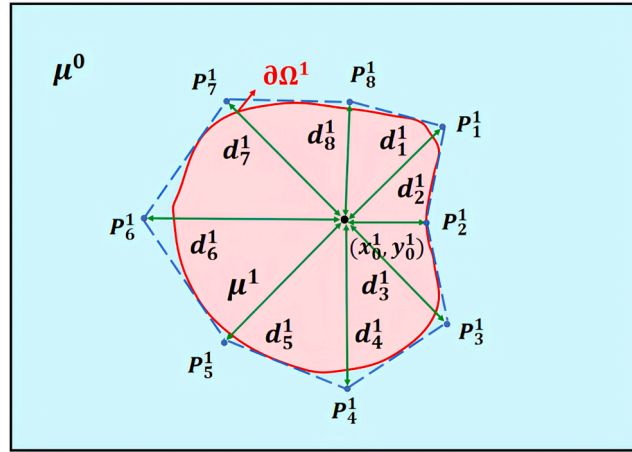
Fig. 3. The nonhomogeneous shear modulus distribution of an inclusion embedded composite.
